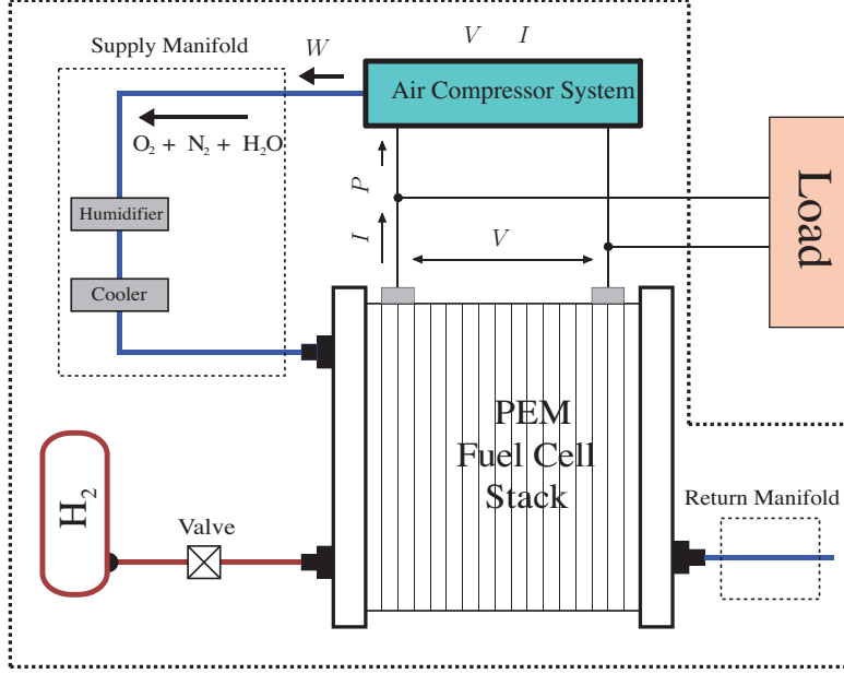
Figure 3: Schematic diagram of the PEMFC-based system
